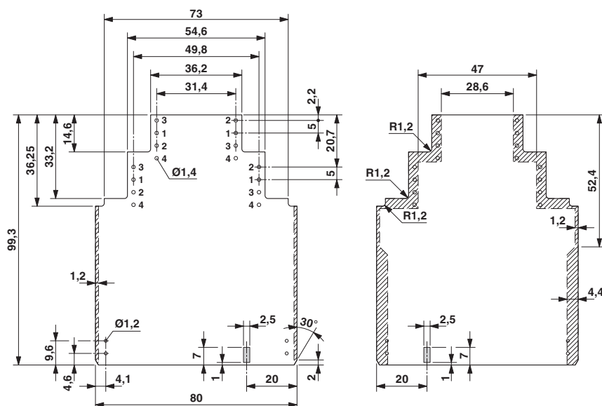
Dimensioned drawing
