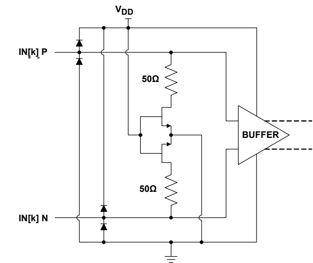
FIGURE 25. CML INPUT EQUIVALENT CIRCUIT FOR THE QLx4600-SL30
