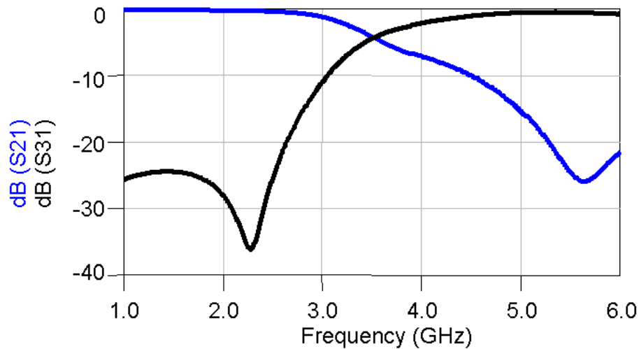
Insertion Loss
