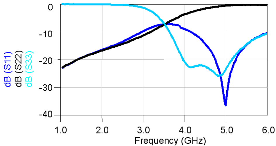
Return Loss
