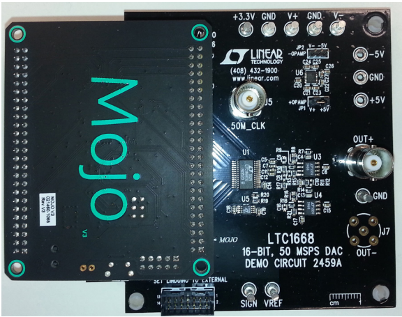
Figure 6. DC2459A Connected to the Mojo Board
