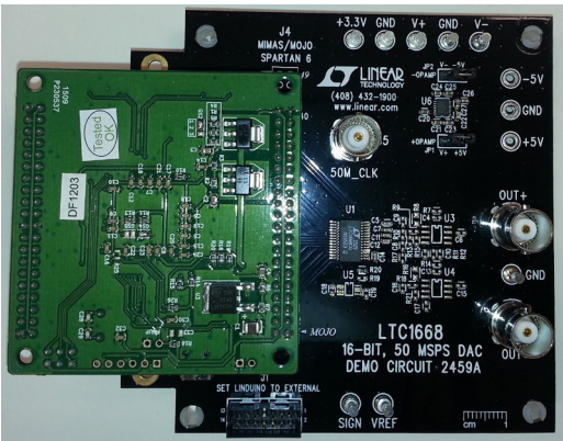
Figure 5. DC2459A Connected to the Mimas Board
