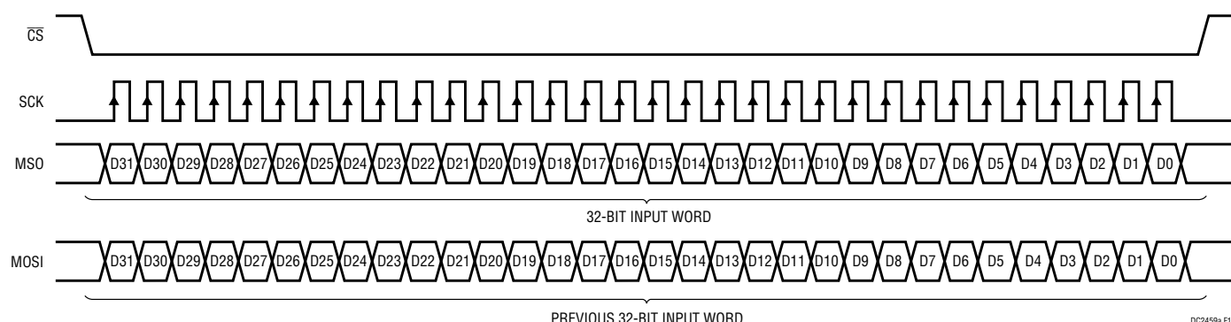
Figure 10. SPI Interface Data Format
