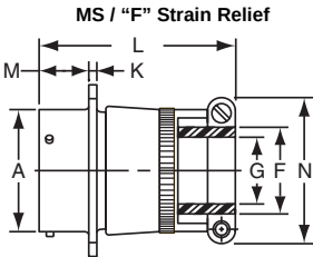
MF00SE-XX-XXX (SR) MS3128F-XX-XXX
