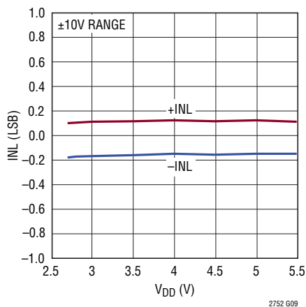
INL vs V_{DD}
