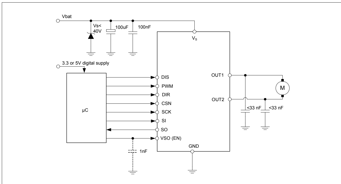
Figure 13 Application Example VSO as Enable Input
