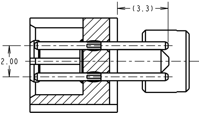
SECTION X-X
