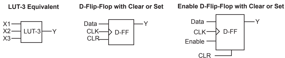
Figure 1-6 • VersaTile Configurations
