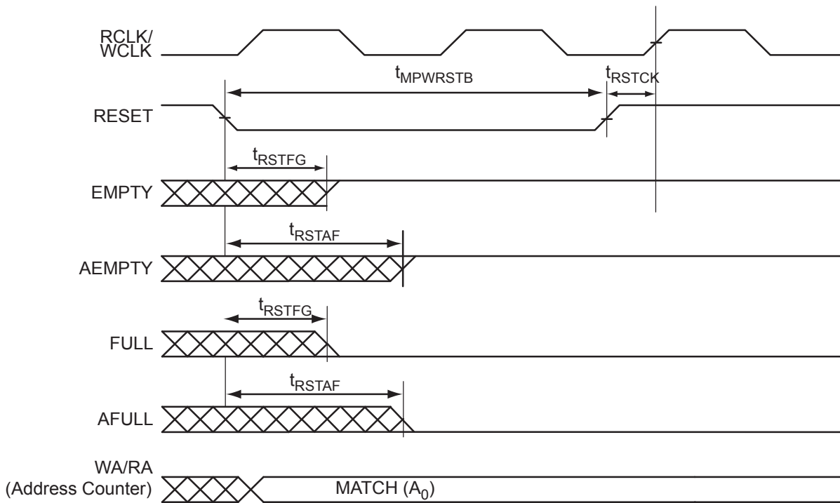
Figure 2-36 • FIFO Reset
