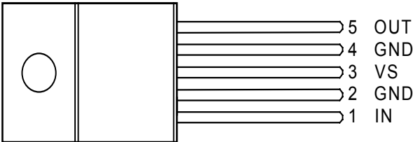
TO-220-5 (T)
