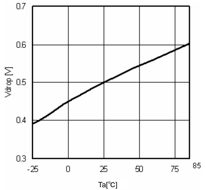
Fig.18 Minimum dropout Voltage 1 (V cc =5V, I o =-1.0A)
