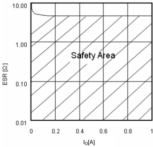
Fig.19 ESR condencer
