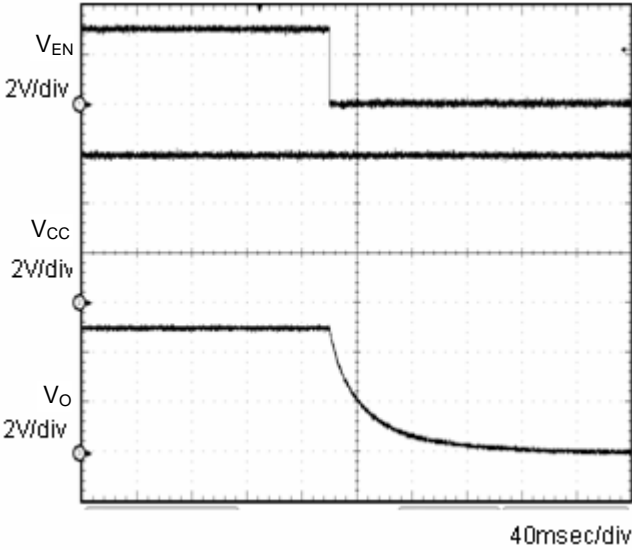
Fig.8 OFF sequence 2 Co=1μF
