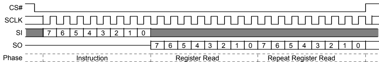
Figure 52. Read Configuration Register (RDCR) Command Sequence
