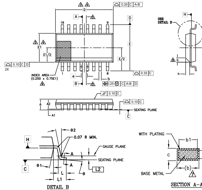
Figure 37. S03016 — 16-Lead Wide Plastic Small Outline Package (300-mil Body Width)
