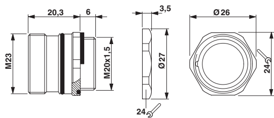
Dimensional drawing
