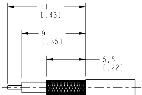
RECOMMENDED CABLE STRIPPING DIM'S. SCALE 3.000
