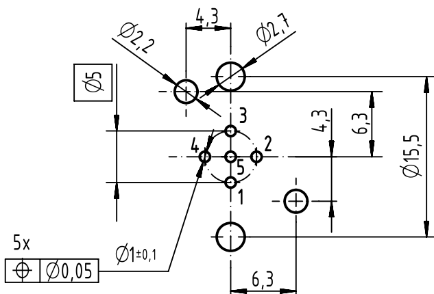
PCB layout
