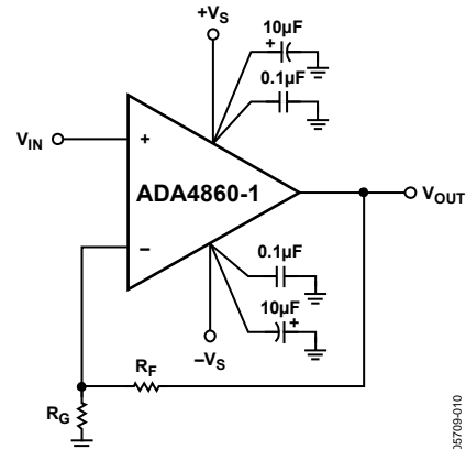
Figure 51. Noninverting Gain
