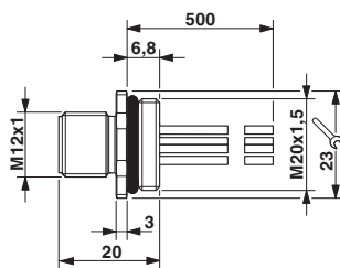
Dimensioned drawing
