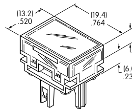
AT4177 Rectangular
