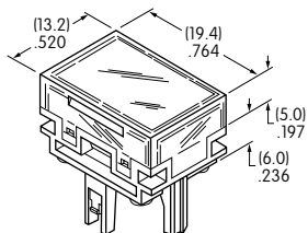
AT4163 Rectangular
