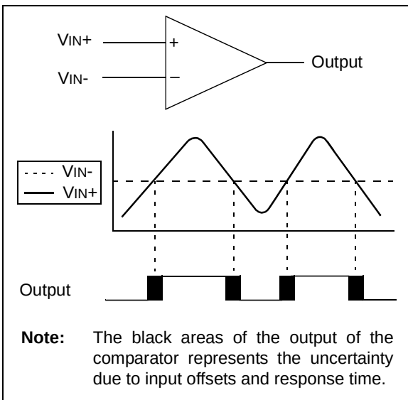
FIGURE 7-1: SINGLE COMPARATOR
