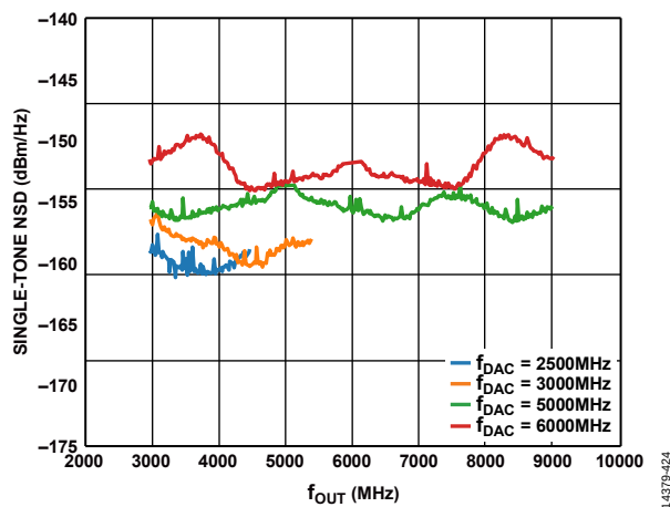
Figure 30. Single-Tone NSD Measured at 70 MHz vs. f_{OUT}
