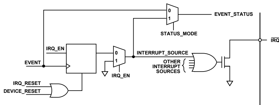
Figure 175. Simplified Schematic of \overline{IRQ} Circuitry
