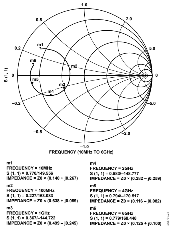
Figure 194. Simulated Smith Chart Showing the DAC Output Impedance ( Z_O = 100 \Omega )
