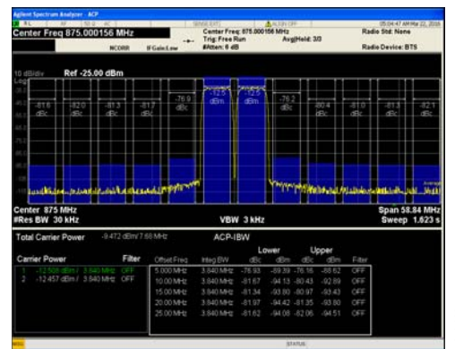
Figure 87. Two-Carrier W-CDMA at 875 MHz
