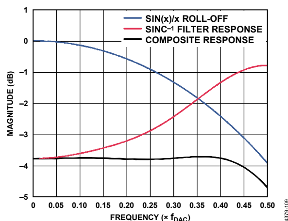
Figure 173. Responses of \text{Sin}(x)/x Roll-Off, the \text{Sinc}^{-1} Filter, and the Composite of the Two
