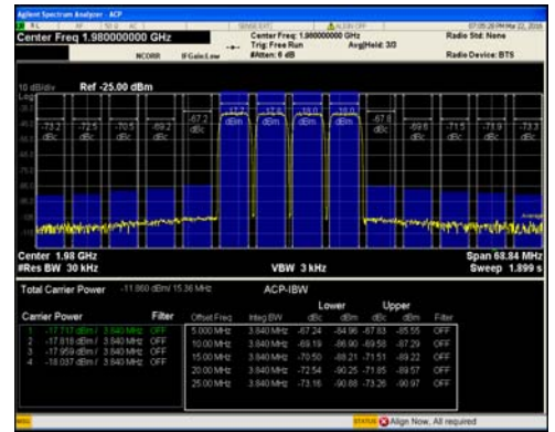
Figure 109. Four-Carrier W-CDMA at 1980 MHz
