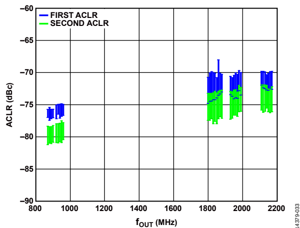
Figure 91. Two-Carrier, W-CDMA ACLR vs. f_{OUT} (First ACLR, Second ACLR)
