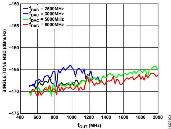
Figure 77. Single-Tone NSD Measured at 70 MHz vs. f_{OUT} over f_{DAC}
