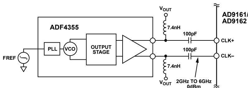
Figure 186. Possible Signal Chain for CLK \pm Input
