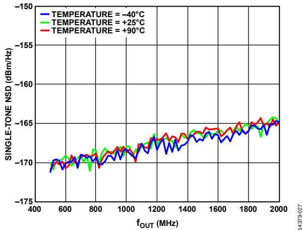
Figure 82. Single-Tone NSD Measured at 70 MHz vs. f_{OUT} over Temperature
