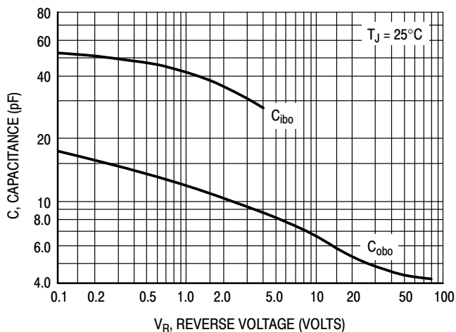
Figure 2. Capacitance
