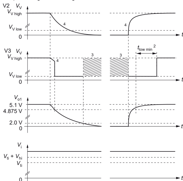
Fig. 26 Relationship between V_i , V_{o1} , V_V , I_V , and V_{o1}/V_{o\ nom} versus time.
