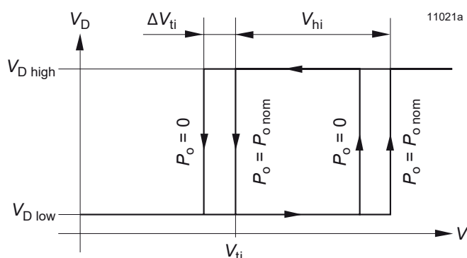
Fig. 22 Definition of V_{ti} , \Delta V_{ti} , and V_{bi} (JFET output)
