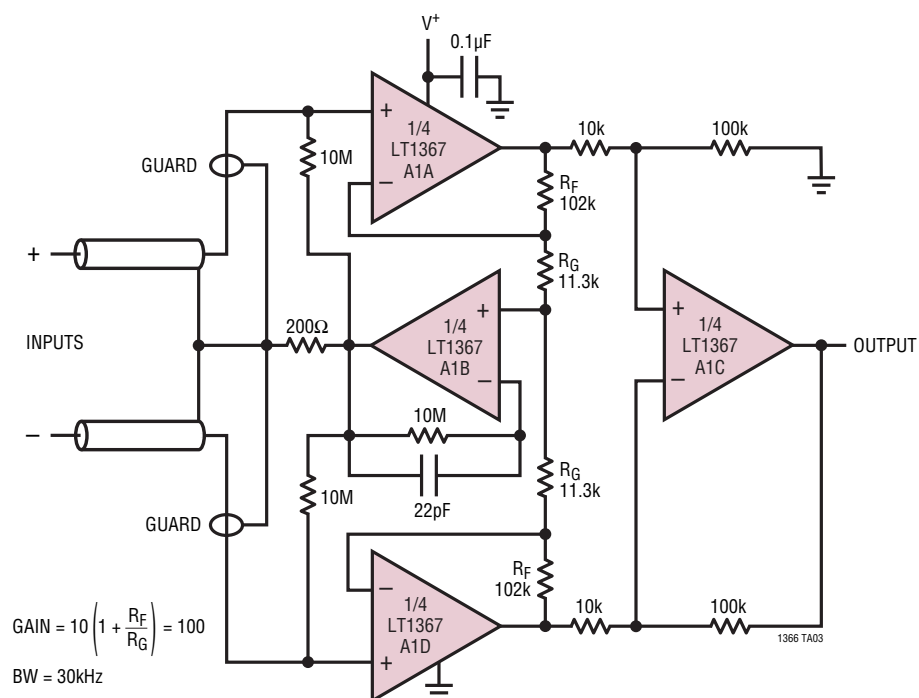
Instrumentation Amplifier
