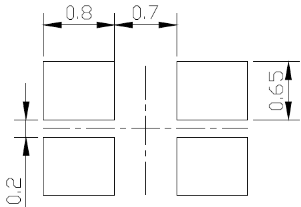
Figure 1. IN-S66TBTRGB Solder Pattern
