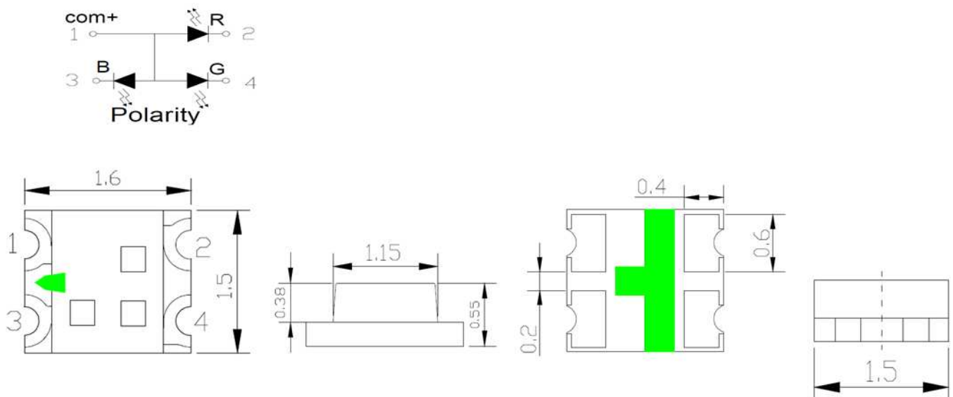
Figure 2. IN-S66TBTRGB Package Dimensions
