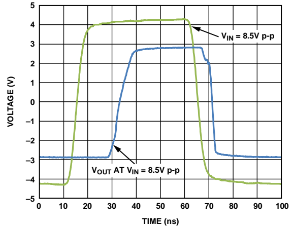
Figure 53. ADV3225 Overdrive Recovery
