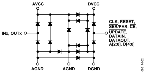
Figure 60. ESD Map
