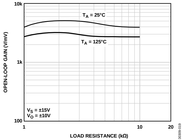
Figure 18. Open-Loop Gain vs. Load Resistance
