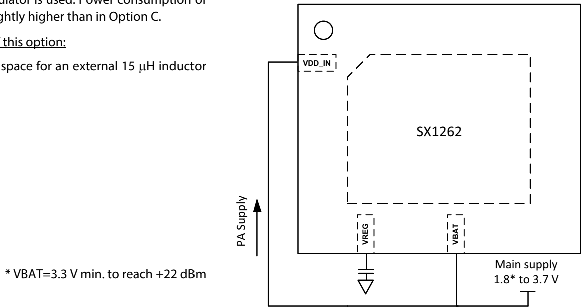
Figure 5-4: SX1262 Diagram with the LDO Regulator Power Option
