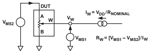
Figure 33. Wiper Resistance
