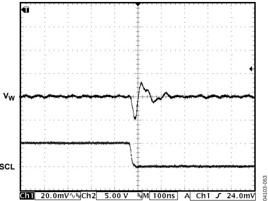
Figure 25. Digital Feedthrough
