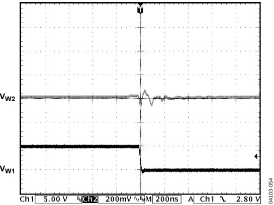
Figure 26. Digital Crosstalk
