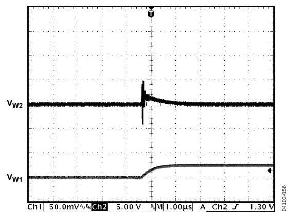
Figure 27. Analog Crosstalk
