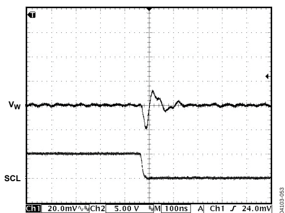
Figure 25. Digital Feedthrough
