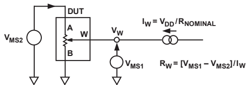
Figure 33. Wiper Resistance
