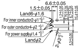
Recommended Board Mounting Pattern
