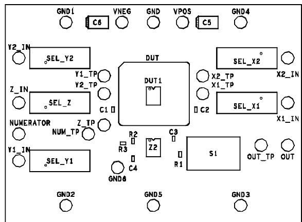
Figure 29. AD633-EVALZ Assembly
