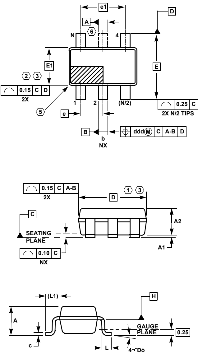
MDP0049 TSOT PACKAGE FAMILY
