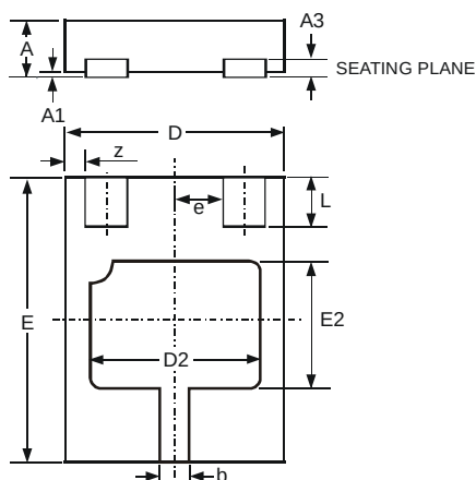
X2-DFN2015-3
