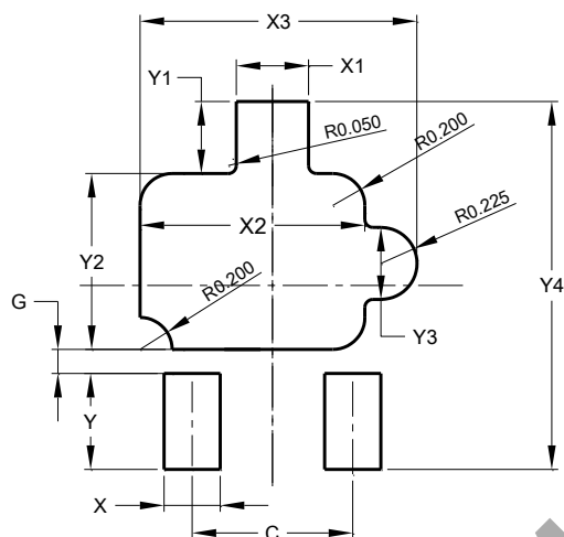
U-DFN2020-3
