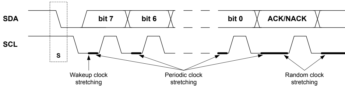
Figure 26-9. Clock Stretching (1)
