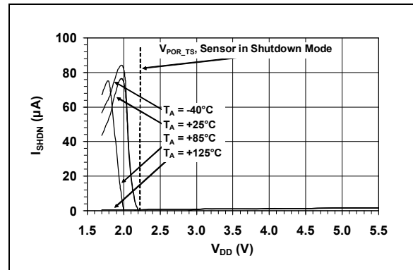
FIGURE 2-15: Shutdown Current vs. V_{DD} .
