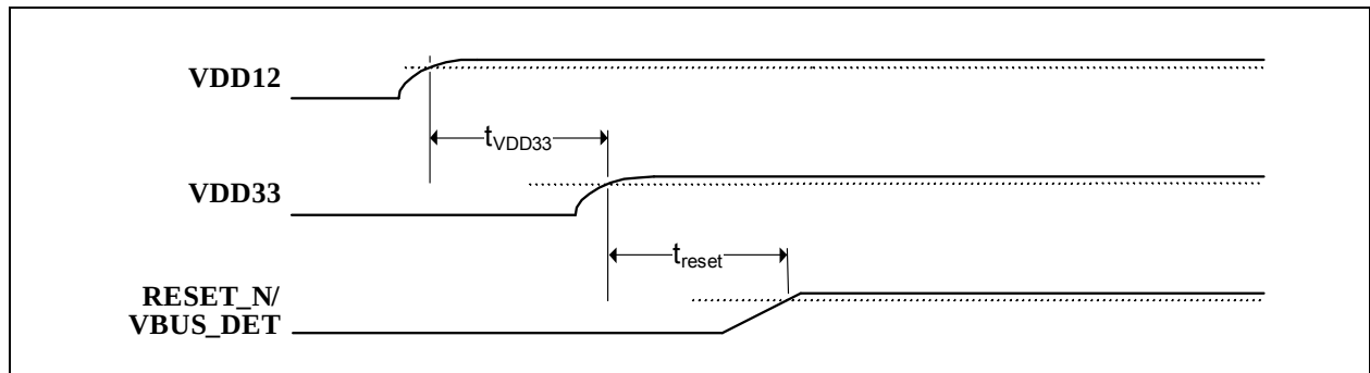
FIGURE 10-2: POWER SUPPLY AND RESET_N SEQUENCE TIMING
