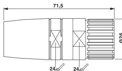
Dimensional drawing
