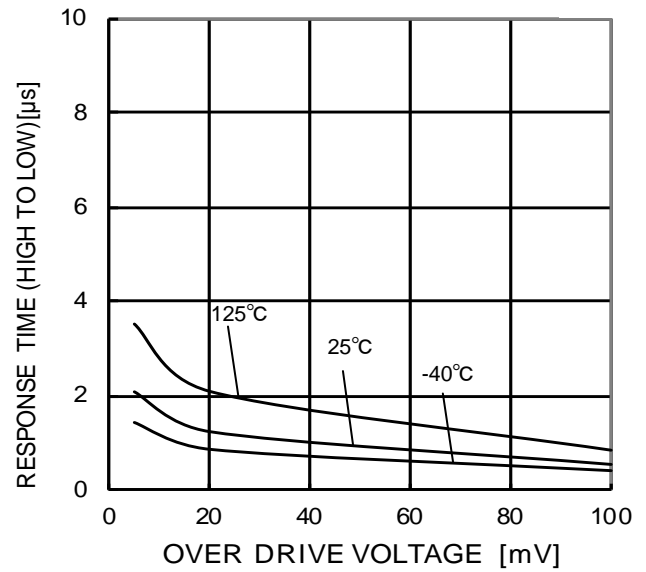
Figure 46. Response Time (High to Low) – Over Drive Voltage (VCC=5V, VRL=5V, RL=5.1k \Omega )
