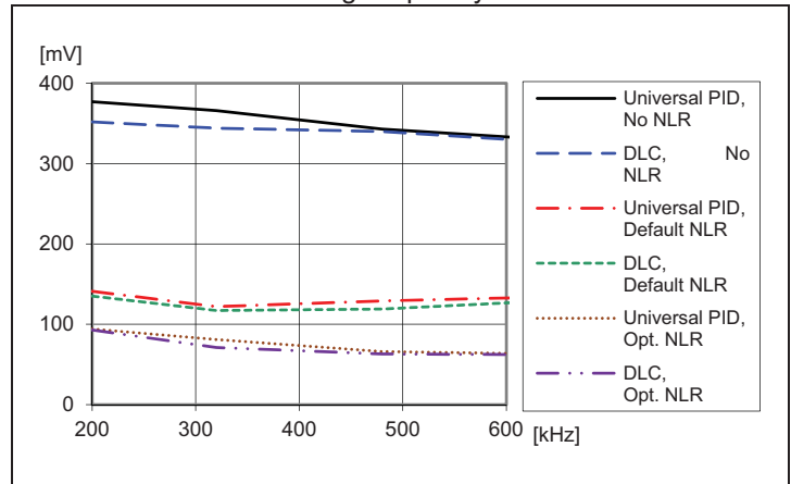
Load transient peak voltage deviation vs. frequency. Step-change (6.25-18.75-6.25 A). T_{P1} = +25\text{ }^{\circ}\text{C} , V_I = 12\text{ V} , V_O = 1.0\text{ V} , C_O = 470\text{ }\mu\text{F}/10\text{ m}\Omega
